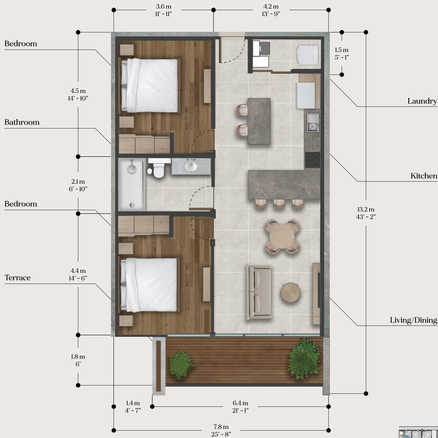
LEVEL 2 - KEY PLAN
